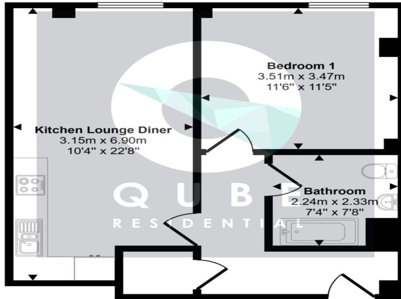
Floorplan
